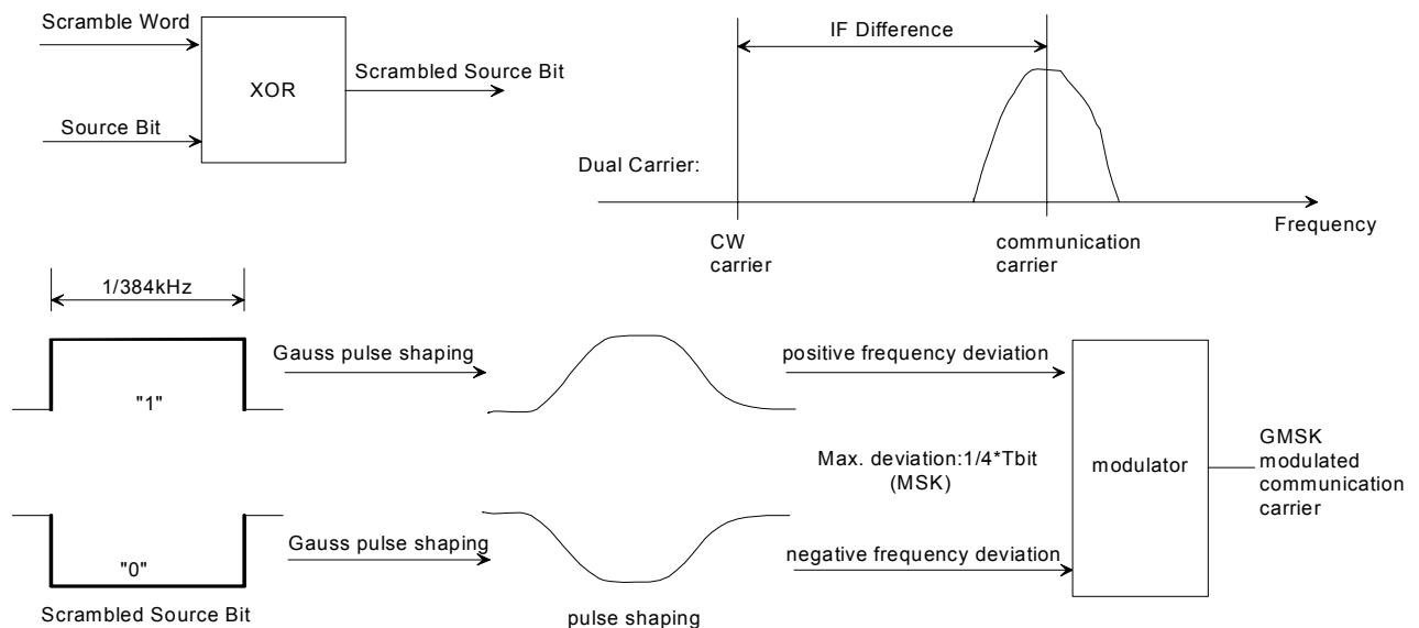
Figure 13 — Forward link modulation and coding
