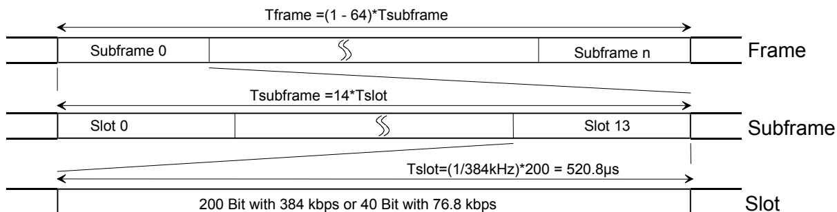
Figure 16 — Frame structure
