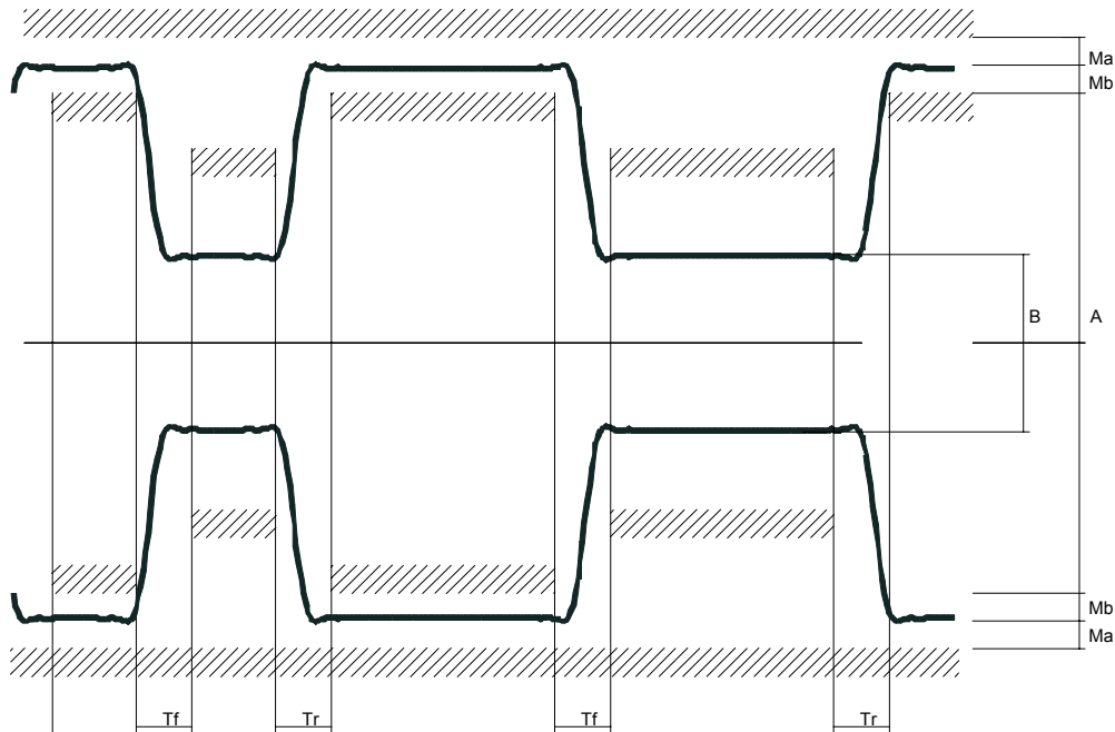
Figure 4 — Example of 40 kbit/s signal
